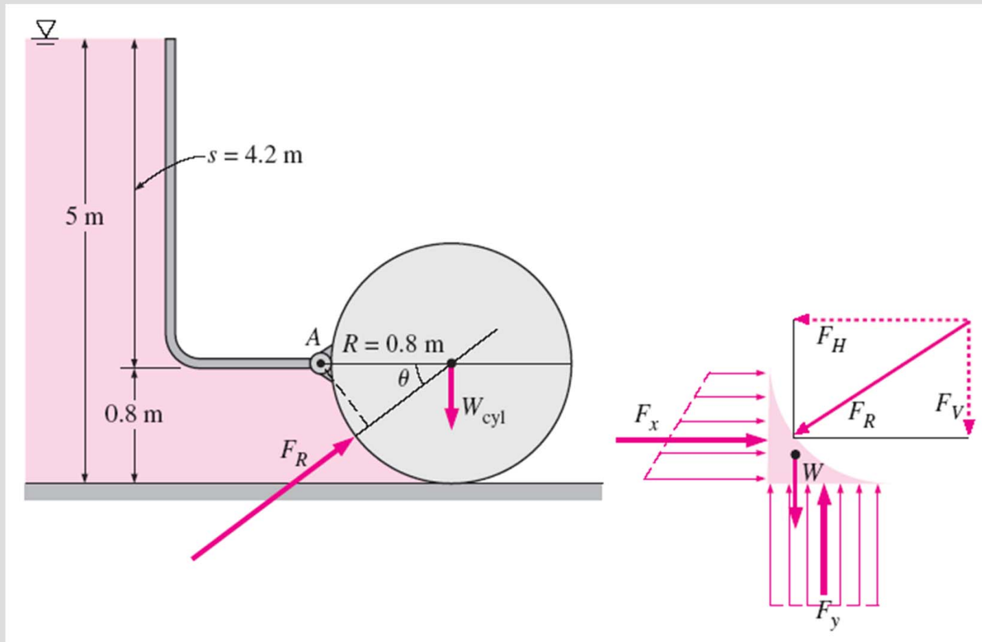
Schematic for Example 3–9 and the free-body diagram of the liquid underneath the cylinder.
